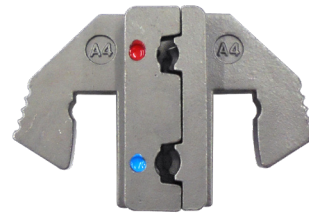
Caméléon Insulated Flag Connector Die A4 (14-22 Awg)
